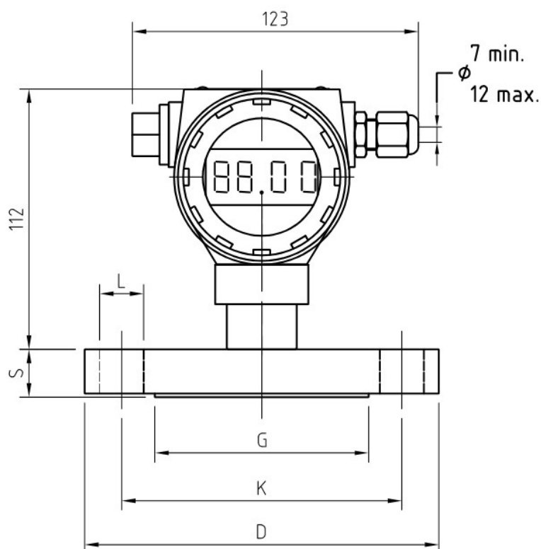
Figure 1 - Attacco flangiato / Flanged connection (UNI, ASME...)
